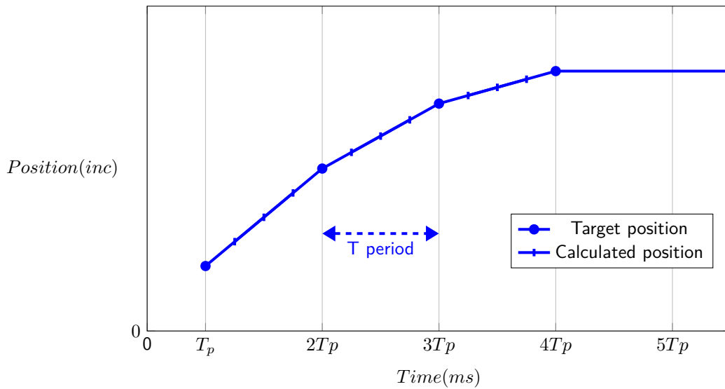
Figure 2.35: Linear interpolation
