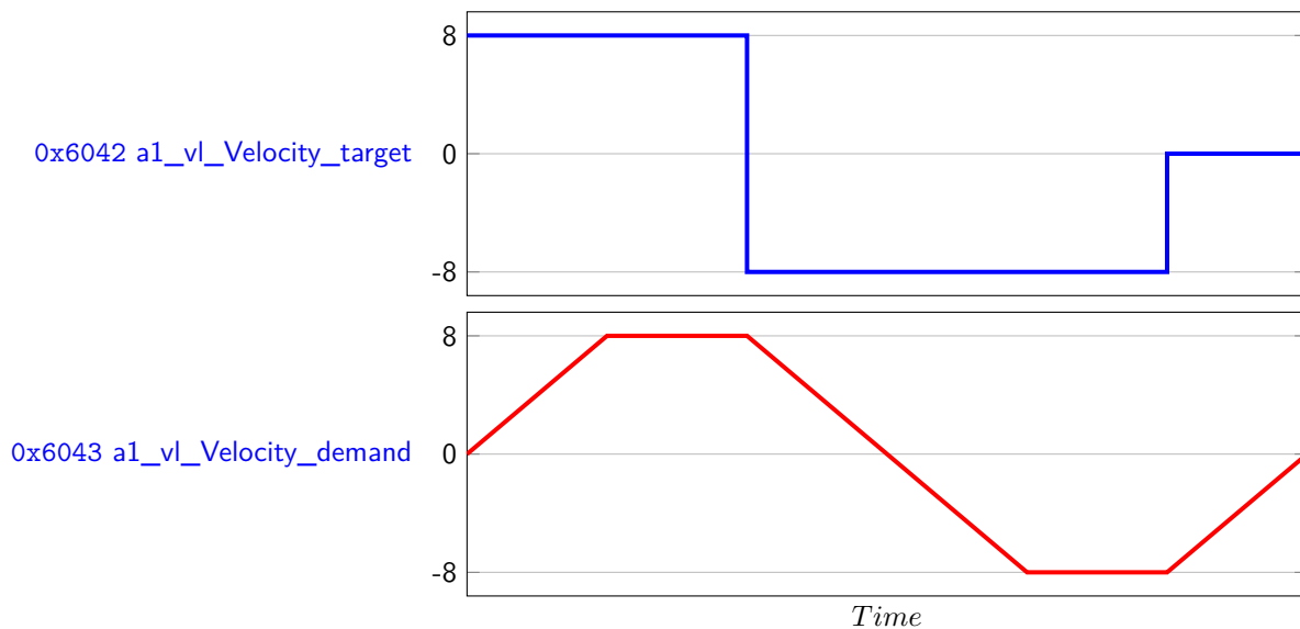
Figure 2.16: Velocity profile
