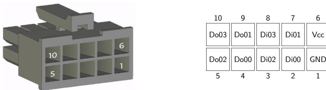
Figure 1.11: J503 pins, 2 x 5 pins, global digital inputs / outputs
