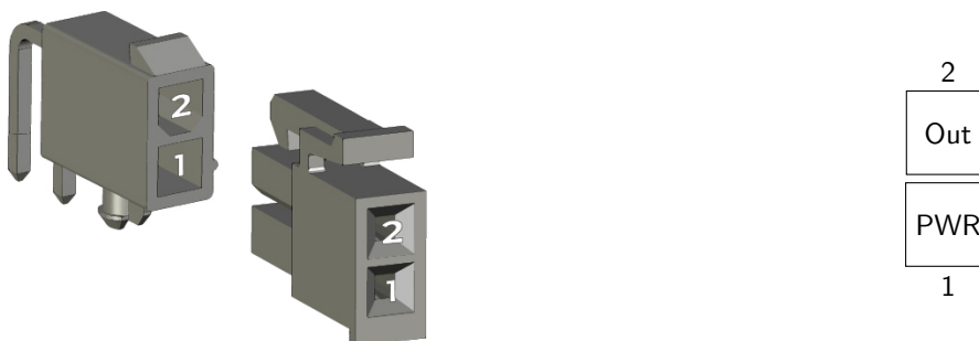
Figure 1.5: J704 pins, 2 pins, brake output
