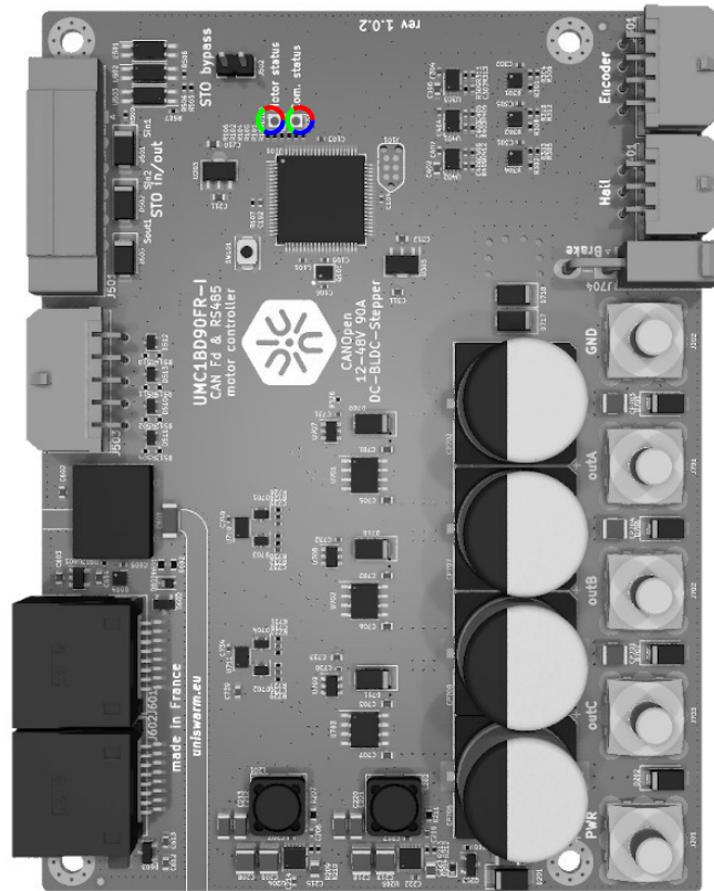
Figure 1.15: UMC1BD90 leds
